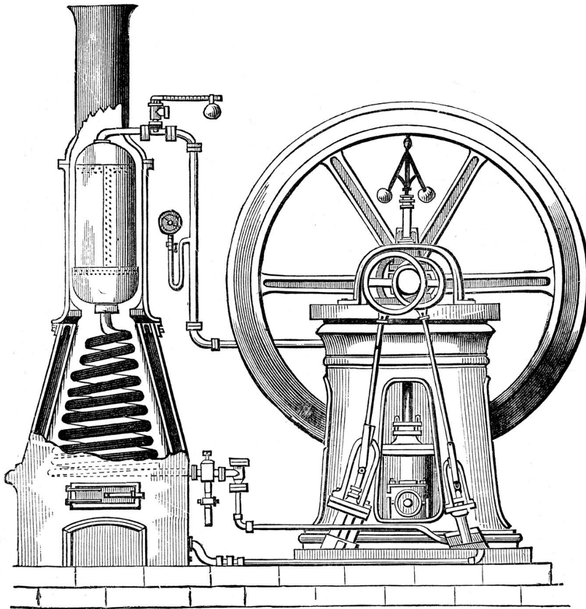
FIG. 8.— Steam Generator.
